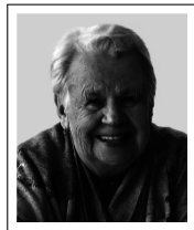
Vera Kublanovskaya, 1920 – 2012
